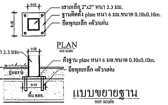
SECTION not scale
